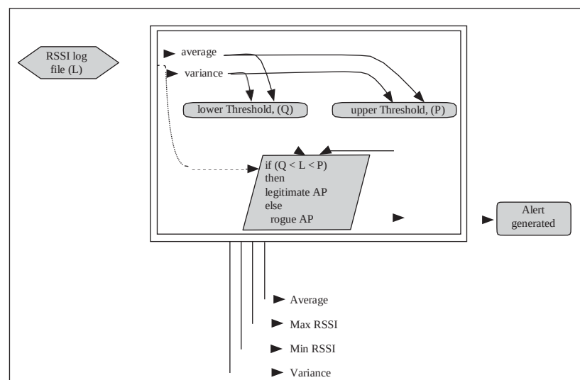
Figure 3.1 The proposed Rogue AP Detection Algorithm (Source: Kamal – Bashah et al. , 2014)
